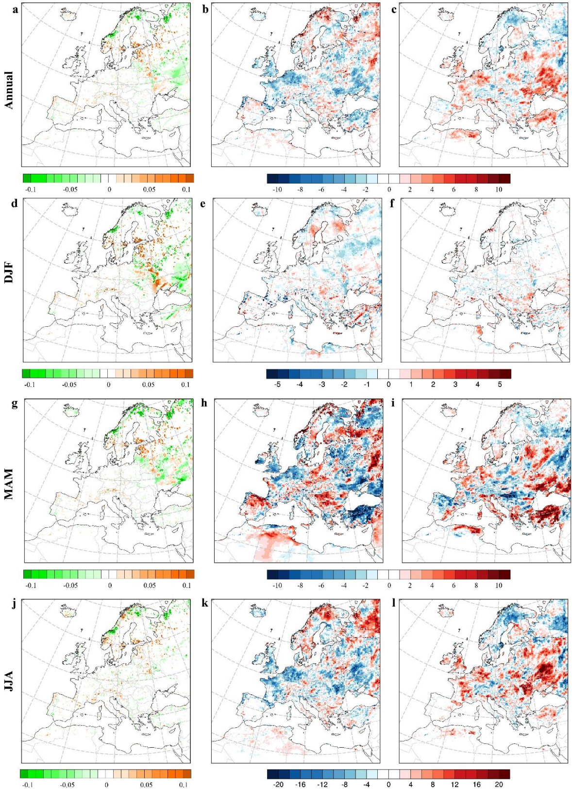
Supplementary Figure 2 Changes in surface albedo (a, d, g, j), sensible heat (b, e, h, k), and latent heat (c, f, i, l) in the annual mean (a, b, c), winter (d, e, f), spring (g, h, i), and summer (j, k, l) in the experiment “LC2015 - LC1992”. Units of sensible and latent heat are W m^{-2} .
