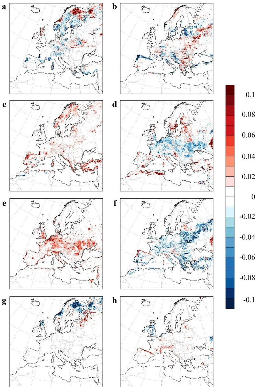
Supplementary Figure 1 Land cover transitions from 1992 to 2015 for the major IGBP land cover classes (LC2015-LC1992). The color bar indicates the fraction of each grid cell where the change occurred. Positive values mean expansion, negative values contraction. Legend: a) evergreen needleleaf forest, b) deciduous broadleaf forest, c) open shrubland, d) cropland, e) urban and built-up, f) cropland/natural vegetation mosaic, g) wetland, h) grassland.
