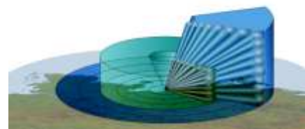
Figure 9: Diagram of a typical 3D-Radar, a mix of vertical electronic beam steering and mechanical horizontal movement of a pencil-beam
