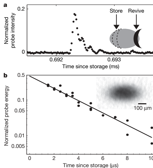
Figure 3 | Light pulse revivals in single clouds. a , A light pulse is revived at the right end of a single BEC of 3.4 \times 10^6 atoms, 0.69 ms after storage in the left end. The cloud was prepared in a harmonic magnetic trap ( \omega_z = 2\pi \times 20 Hz, \omega_r = 2\omega_z ). All light parameters are similar to those in Fig. 2. b , Decay of revival signal in thermal cloud. The energy of the revived light pulse is plotted as a function of time since pulse storage. The thermal cloud (inset) has 13.5 \times 10^6 atoms at 470 nK, just above the critical temperature for BEC (340 nK) in the trap described in a . Input probe Rabi frequency is 2\pi \times 3.2 MHz; coupling storage and revival Rabi frequencies are 2\pi \times 3.5 and 2\pi \times 17.5 MHz, respectively.
