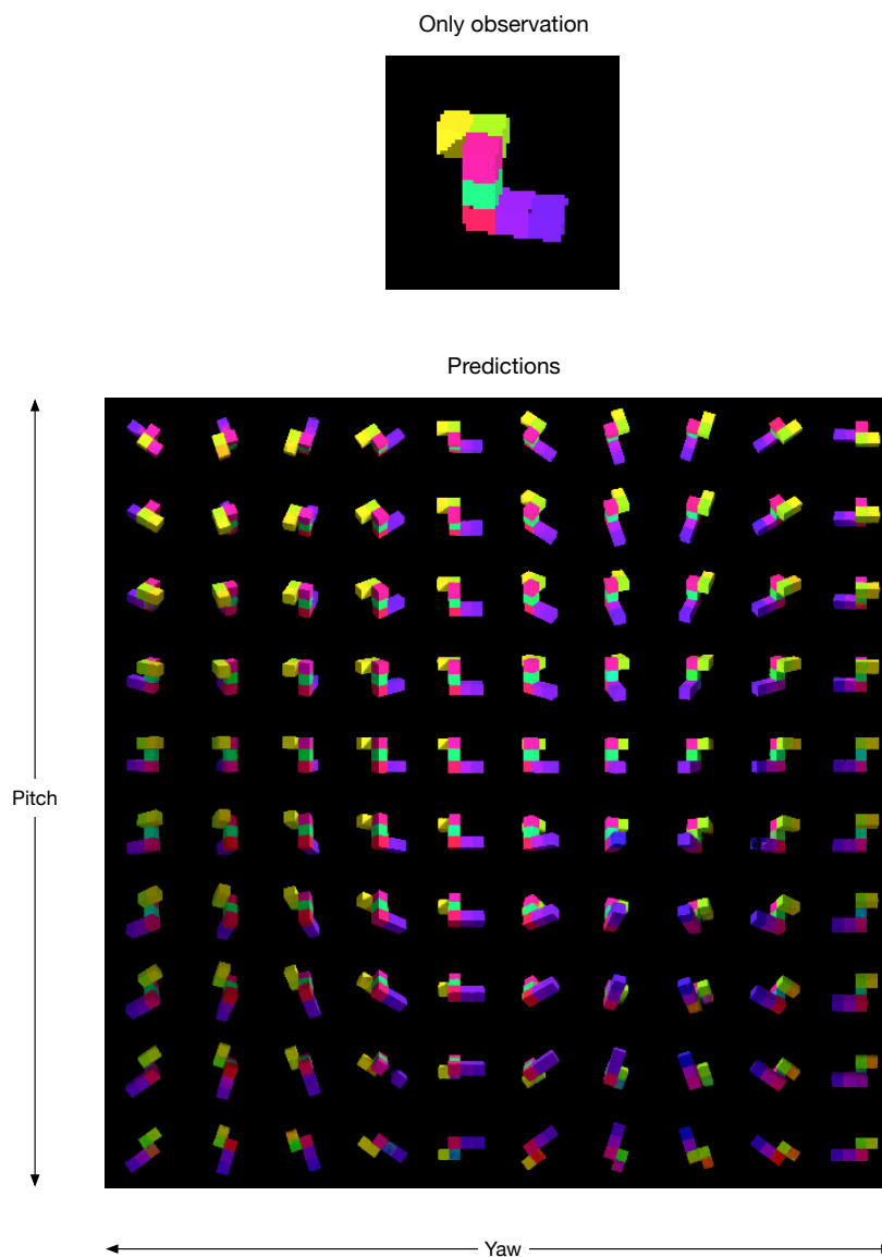
Figure S9: Shepard-Metzler environment . Given a single observation of a test object, the representation network produces a neural description of it. The generator is capable of predicting accurate images from arbitrary query viewpoints. This implies that the scene description accurately captures the positions and colours of multiple parts that make up the object. The model’s predictions are consistent with occlusion, lighting and shading, and are typically indistinguishable from ground-truth.
