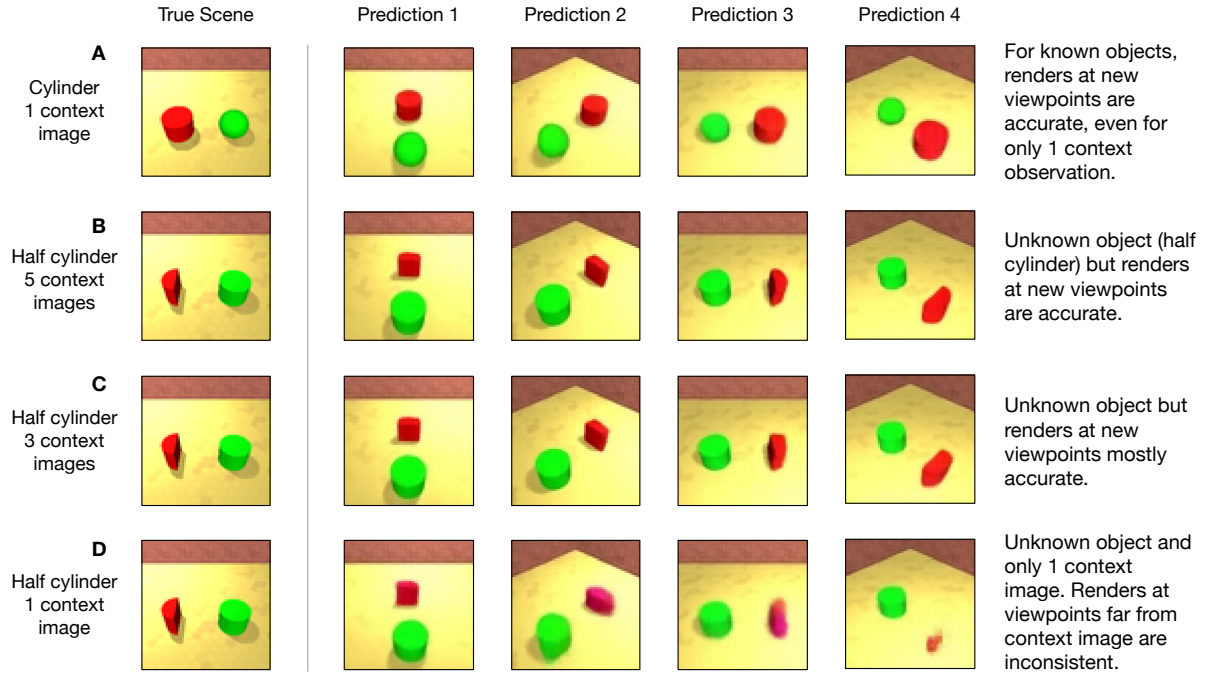
Figure S14: Relationship between generalisation and number of context observations. We observe that the GQN’s ability to generalise to out-of-distribution scenes is affected by the number of context images it is allowed to use to compute the scene representation. (A) With only a single observation, the model successfully renders a familiar object from new viewpoints. (B) With 5 context observations, the model successfully renders an out-of-distribution object (half-cylinder) from new viewpoints. As the number of context images is reduced (C-D), the model’s renders become progressively less consistent. The renders are most accurate from viewpoints that are closest to the context observations’ viewpoints.
