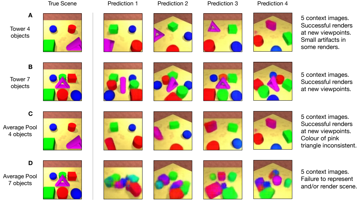
Figure S16: Generalisation to scenes with more objects than trained. We train GQNs on up to 3 objects as before; here, however, we test their performance on a number of strongly out-of-distribution scenes with 4 or 7 objects each. The tower architecture (see Fig. S1) is capable of generalising to 4 ( A ) and 7 ( B ) objects. The average pool architecture is mostly accurate on ( C ) 4 objects, however performance degrades with ( D ) 7 objects. The tower architecture’s superior performance is due to the spatial nature of its scene representation. By contrast, the average pool architecture’s non-spatial representation appears to bind object properties in a manner which is dependent on the number of objects in the scene, resulting in poor extrapolation to scenes with more objects than trained.
