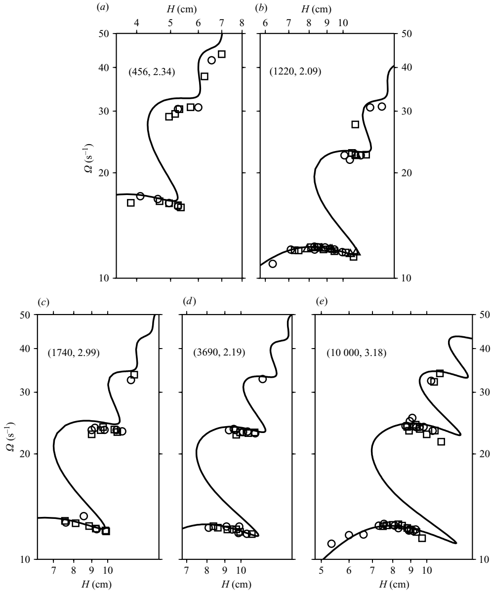
FIGURE 12. Comparison of experimentally measured (symbols) and numerically predicted (solid lines) frequencies as functions of height for the Zanja experiments. The fluid viscosity was \nu = 300 \text{ cm}^2 \text{ s}^{-1} for experiment (a) and 1000 \text{ cm}^2 \text{ s}^{-1} for experiments (b)–(e). Values of (\Pi_1, \Pi_2) for each experiment are indicated in parentheses. Measurements were obtained in series with H increasing (squares), decreasing (circles), and varied randomly (triangles.) Error bars on H are smaller than the size of the symbols. Error bars on \Omega , which in most cases do not exceed \pm 5\% , have been omitted for clarity.
