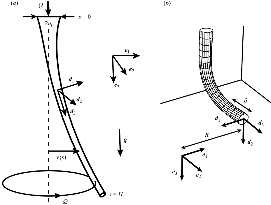
FIGURE 7. Geometry of liquid rope coiling in the inertio-gravitational regime. \mathbf{e}_i ( i = 1, 2, 3 ) are Cartesian unit vectors fixed in a frame rotating with the rope, and \mathbf{d}_i are orthogonal material unit vectors defined at each point on its axis, \mathbf{d}_3 being the tangent vector. The parameters Q , a_0 , H , R and \Omega are defined as in figure 1. (a) Geometry of the tail, modelled as an extensible string with negligible resistance to bending and twisting. This string lies in the plane normal to \mathbf{e}_2 , and \mathbf{d}_1 \cdot \mathbf{e}_2 = 0 . The lateral displacement of the axis from the vertical is y(s) , where s is the arclength measured from the injection point. (b) Geometry of the rope near the contact point. Bending and twisting are important in a boundary layer of arcwise extent \delta near this point. Right at the contact, \mathbf{d}_1 is horizontal and points towards the center of the circle (of radius R ) along which the rope is laid down.
