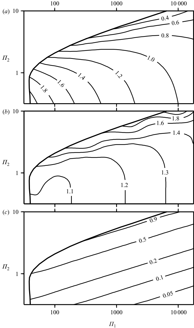
FIGURE 4. Contours of (a) height H_1(g/\nu^2)^{1/3} , (b) frequency \Omega_1(\nu/g^2)^{1/3} , and (c) thinning factor a_1/a_0 at the first turning point in the curve of frequency vs. height. Dimensionless groups \Pi_1 and \Pi_2 are defined by (2.1).
