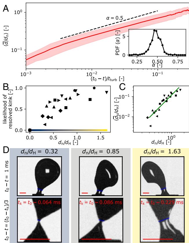
Fig. 4. Role of the turbulence in kink formation. (A) Ensemble average of the normalized average neck diameter \langle \bar{d} \rangle / d_n over all experiments for various needles and levels of turbulence, with the time until pinch-off normalized by the turbulent timescale at the needle length scale, t_{\text{turb}} = (d_n^2 / \epsilon)^{1/3} . The shaded area indicates the standard deviation, and the black line indicates the \alpha = 1/2 inertial power law scaling. Inset shows the distribution of the exponent \alpha obtained by fitting \bar{d} \propto (t_0 - t)^\alpha for each experiment ( Materials and Methods ). The distribution is centered around 0.5. (B) The portion of cases with a resolved kink at each experimental condition as a function of d_n / d_H , with kinks rarely appearing at low d_n / d_H but almost always being resolved as the ratio approaches 1. (C) The neck size when the kink appears, d_k , as a function of d_n / d_H , which exhibits a power law relation \langle \bar{d}_k \rangle / d_H \sim (d_n / d_H)^\beta , with \beta = 2.1 obtained by a fit (which is shown in green). (D) Snapshots of the bubble at t_0 - t = 1 ms ( Upper ) and 2/3 of the way between kink formation and pinch-off ( Lower ) for cases at 3 different d_n / d_H , with the background shading mapped to the color bar in B. When d_n / d_H increases, larger initial deformations lead to earlier and larger kink formation. (Scale bar: 1 mm.)
