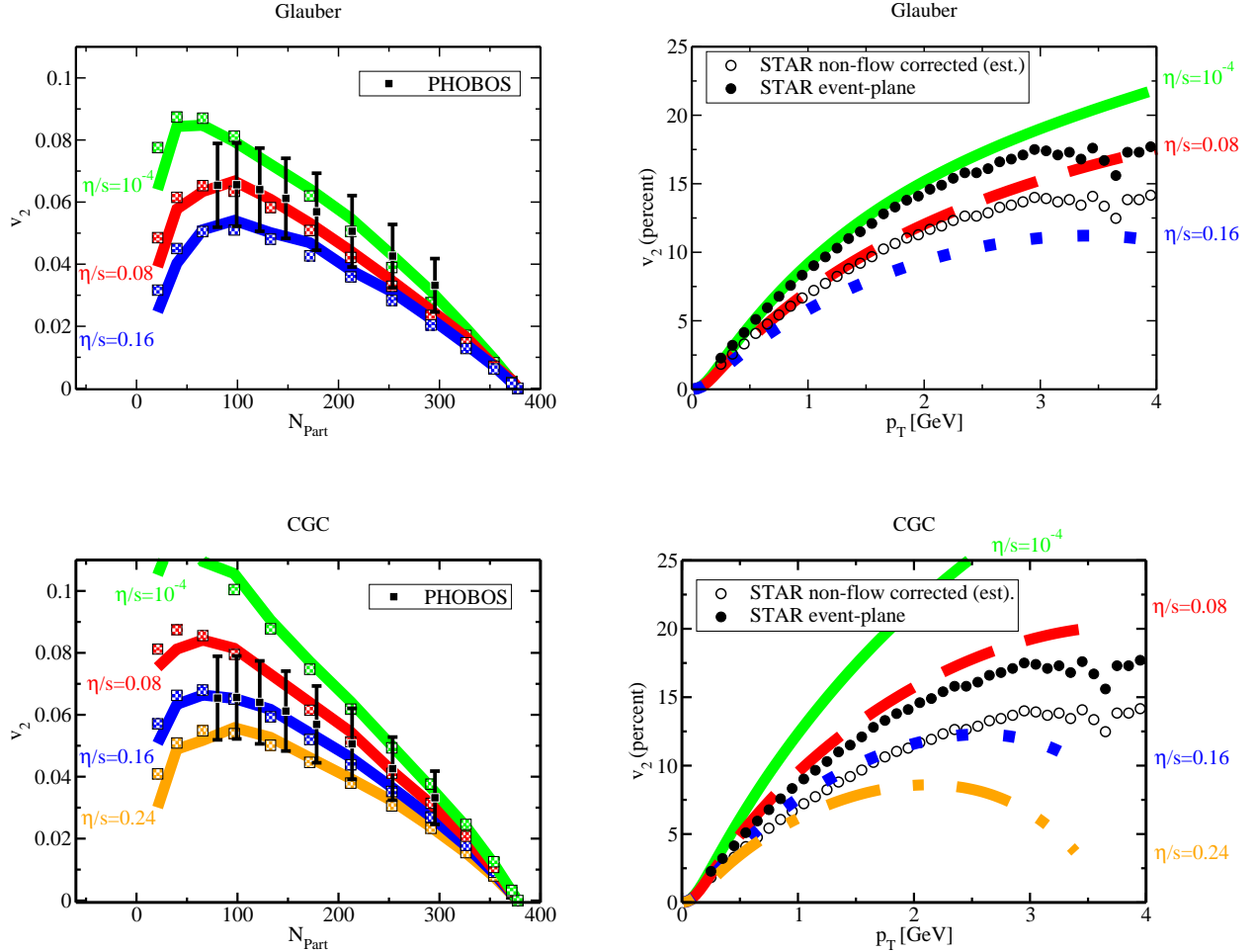
FIG. 8: (Color online) Comparison of hydrodynamic models to experimental data on charged hadron integrated (left) and minimum bias (right) elliptic flow by PHOBOS [85] and STAR [87], respectively. STAR event plane data has been reduced by 20 percent to estimate the removal of non-flow contributions [87, 88]. The line thickness for the hydrodynamic model curves is an estimate of the accumulated numerical error (due to, e.g., finite grid spacing). The integrated v_2 coefficient from the hydrodynamic models (full lines) is well reproduced by \frac{1}{2}e_p (dots); indeed, the difference between the full lines and dots gives an estimate of the systematic uncertainty of the freeze-out prescription.
