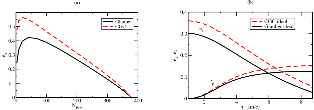
FIG. 4: (Color online) Left: The initial spatial anisotropy for the Glauber and CGC model. Right: The time evolution of the spatial and momentum anisotropy for a collision with b = 7 fm in ideal hydrodynamics.
