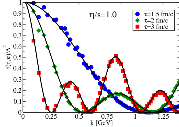
FIG. 3: (Color online) The correlation function f(\tau, \mathbf{k}) as a function of momentum k = |\mathbf{k}| for a lattice with a = 1 \text{ GeV}^{-1} , 64^2 sites and averaged over 30 initial configurations (symbols), compared to the result from the linearized hydrodynamic equations (lines).
