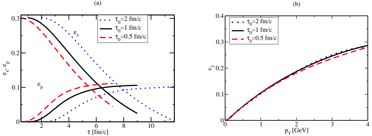
FIG. 9: (Color online) Momentum anisotropy (a) and elliptic flow for charged hadrons (b) for b = 7 fm, \eta/s = 0.08 and different hydrodynamic initialization times \tau_0 . Horizontal light gray lines in (a) are visual aids to compare the final value of e_p . As can be seen from these plots, neither the final e_p nor the charged hadron v_2 depend sensitively on the value of \tau_0 if the same energy distribution is used as initial condition at the respective initialization times. Simulation parameters were T_i = 0.29 GeV, T_f = 0.14 GeV for \tau_0 = 2 fm/c, T_i = 0.36 GeV, T_f = 0.15 GeV for \tau_0 = 1 fm/c, and T_i = 0.43 GeV, T_f = 0.16 GeV for \tau_0 = 0.5 fm/c.
