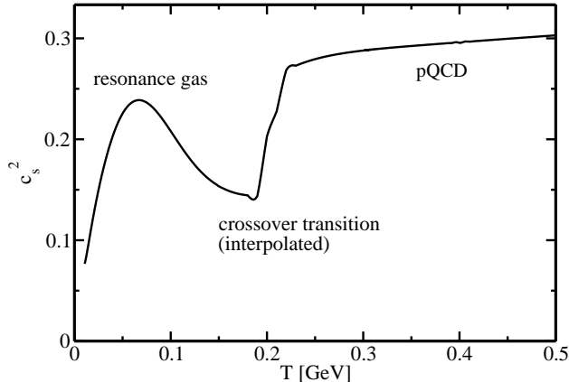
FIG. 1: The speed of sound squared from Ref. [55], used in the hydrodynamic simulations. See text for details.
