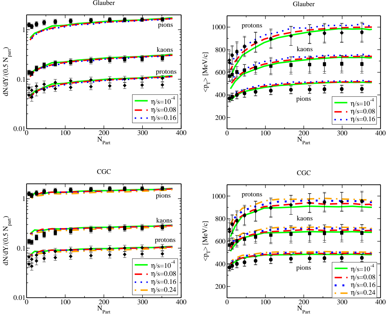
FIG. 7: (Color online) Centrality dependence of total multiplicity dN/dY and \langle p_T \rangle for \pi^+, \pi^-, K^+, K^-, p and \bar{p} from PHENIX [84] for Au+Au collisions at \sqrt{s} = 200 GeV, compared to the viscous hydrodynamic model and various \eta/s , for Glauber initial conditions and CGC initial conditions. The model parameters used here are \tau_0 = 1 fm/c, \tau_{II} = 6\eta/s , \lambda_1 = 0 , T_f = 140 MeV and adjusted T_i (see Table I).
