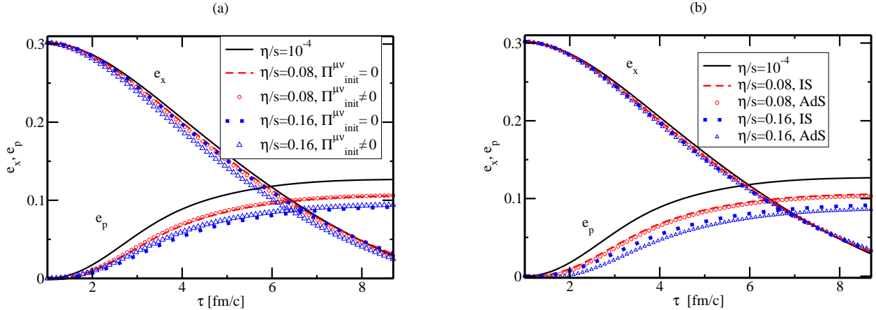
FIG. 5: (Color online) Spatial and momentum anisotropy for the Glauber model at b = 7 fm with T_i = 0.353 GeV, \tau_0 = 1 fm/c and various values for the viscosity (grid spacing a = 2 GeV ^{-1} ). (a): The dependence on the initialization value of the shear tensor: shown are results for vanishing initial value ( \Pi_{\text{init}}^{\mu\nu} = 0 ) and Navier-Stokes initial value ( \Pi_{\text{init}}^{\mu\nu} \neq 0 ), given in Eq. (9). (b): The dependence on the choice of value for \tau_{\Pi} , \lambda_1 : shown are results for \tau_{\Pi} = \frac{6}{T} \frac{\eta}{s} , \lambda_1 = 0 (labelled “IS”) and \tau_{\Pi} = \frac{2(2-\ln 2)}{T} \frac{\eta}{s} , \lambda_1 = \frac{\eta}{2\pi T} (labelled “AdS”). For \tau_{\Pi} = \frac{2(2-\ln 2)}{T} \frac{\eta}{s} , the results for \lambda_1 = 0 (not shown) would be indistinguishable by bare eye from those for \lambda_1 = \frac{\eta}{2\pi T} .
