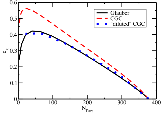
FIG. 10: (Color online) Spatial eccentricity for the Glauber and CGC model compared to evolving the CGC model according to Eq.(48) for \tau = 1.5 fm/c. This implies that starting with Glauber-type initial conditions at \tau_0 > 1 fm/c may not be unreasonable.
