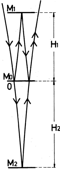
FIG. 1. Schematic diagram of an interferometer with only horizontal mirrors M_0 , M_1 , M_2 , which would be suitable for detecting gravitational effects using ultracold neutrons.
