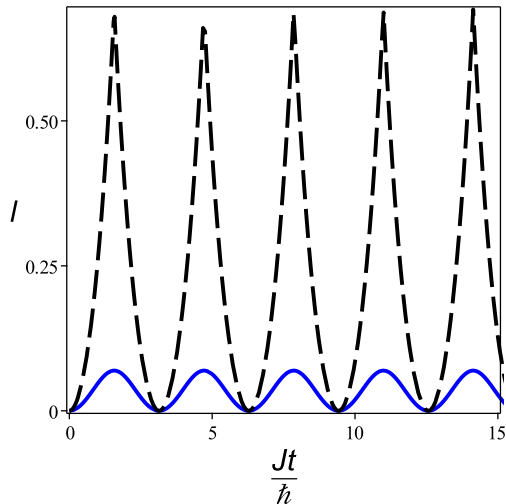
FIG. 2: (Color online) Time dependence of the density of the return probability l(t) of the transverse Ising chain for H_1 = 0 and H_0 = 0.5H_c (blue solid line) and H_0 = 3H_c (black dashed line).
