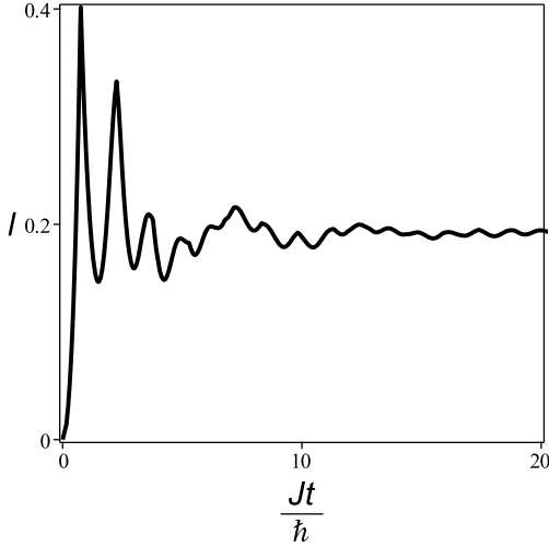
FIG. 5: Time dependence of the density of the return probability l(t) of the XY spin-1/2 chain for H_1 = 1.5H_c and H_0 = 2H_c , \gamma_0 = -5 and \gamma_1 = 1 .
