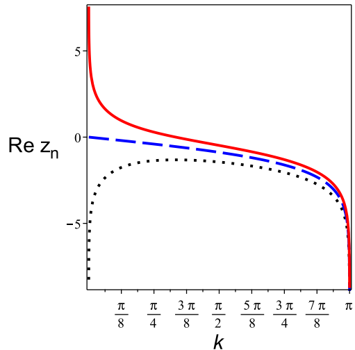
FIG. 1: (Color online) Dependence of \text{Re}z_n of the transverse Ising chain on the wave vector k for H_1 = 0 and H_0 = 0.5H_c (black dotted line), H_0 = H_c (blue dashed line), and H_0 = 2H_c (red solid line).
