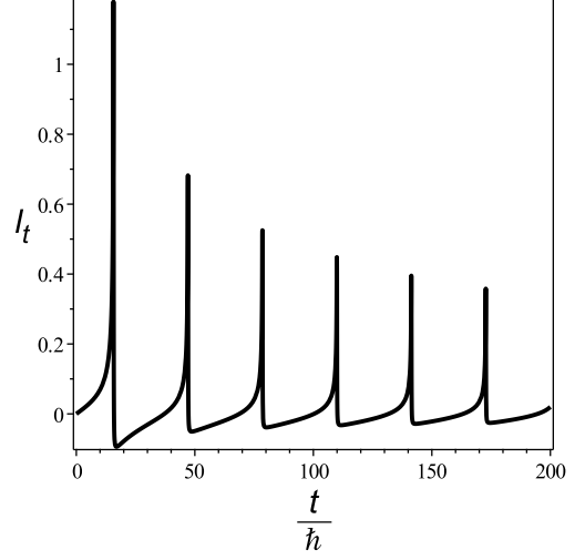
FIG. 9: Time dependence of the time derivative l_t of the density of the return probability l_t of the XX spin-1/2 chain. The parameters are the same as in Fig. 8.
