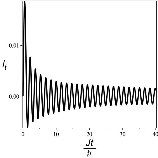
FIG. 6: Time dependence of the density of the return probability l(t) of the XX spin-1/2 chain for \mu_1 = -\mu_2 , and 2\mu_1 H_0 = 0.1J and H_1 = 0 .
