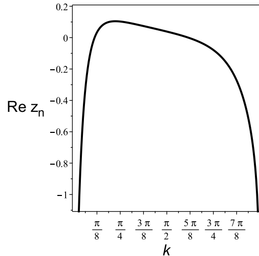
FIG. 4: Dependence of \text{Re} z_n of the XY spin-1/2 chain on the wave vector k for H_1 = 1.5H_c and H_0 = 2H_c , \gamma_0 = -5 and \gamma_1 = 1 .
