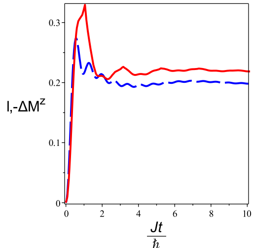
FIG. 10: (Color online) Time dependence of the density of the return probability l(t) (red solid line) and the change of the magnetization \Delta M^z (blue dashed line) of the transverse field Ising chain (at T = 0.01 ) for J = 2 , H_0 = 0 and H_1 = -1.5 (without quantum quench across the quantum critical point H_c = J ).
