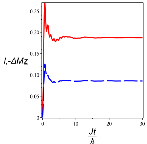
FIG. 10: (Color online) Time dependence of the density of the return probability l(t) (red solid line) and the change of the magnetization \Delta M^z (blue dashed line) of the transverse field Ising chain (at T = 0.01 ) for J = 2 , H_0 = 0 and H_1 = -1.5 (without quantum quench across the quantum critical point H_c = J ).
