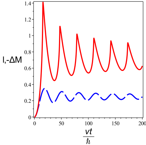
FIG. 12: (Color online) The same as in Fig. 10, and 11 but for H_1 = -2.1 .
