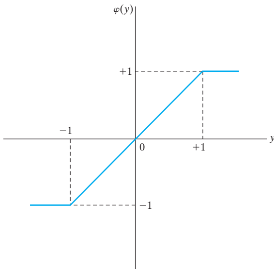
FIGURE 13.16 Piecewise-linear activation function used in the BSB model.
