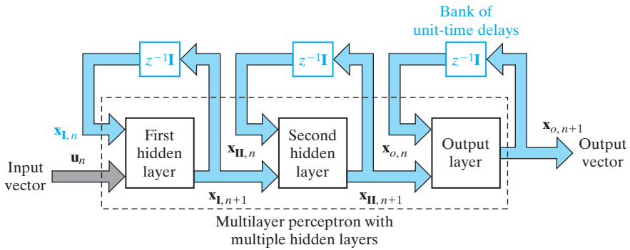
FIGURE 15.4 Recurrent multilayer perceptron; feedback paths in the network are printed in red.
