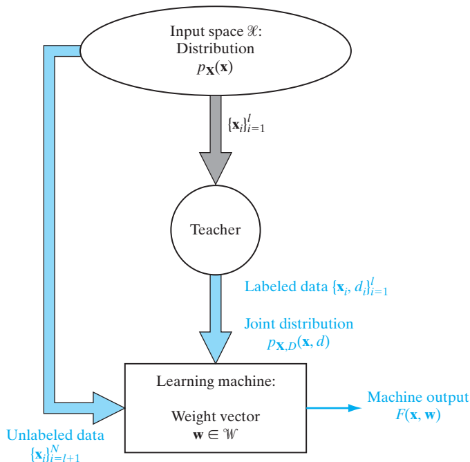
FIGURE 7.4 Model of the semisupervised learning process.
