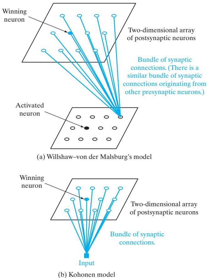
FIGURE 9.1 Two self-organized feature maps.
