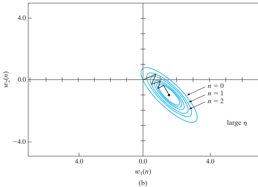
FIGURE 3.2 Trajectory of the method of steepest descent in a two-dimensional space for two different values of learning-rate parameter: (a) small \eta (b) large \eta . The coordinates w_1 and w_2 are elements of the weight vector \mathbf{w} ; they both lie in the \mathcal{W} -plane.
