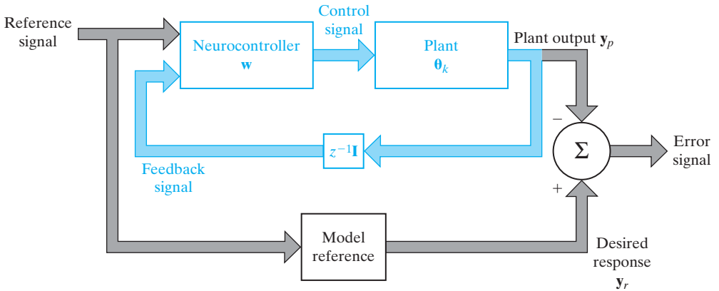
FIGURE 15.18 Model-reference adaptive control system; the feedback loop of the system is printed in red.
