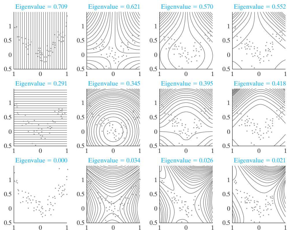
FIGURE 8.13 Two-dimensional example illustrating kernel PCA. From left to right, the polynomial degree of the kernel is d = 1, 2, 3, and 4, respectively. From top to bottom, the first three eigenvectors in the feature space are shown. The first column corresponds to linear PCA, and the other three columns correspond to kernel PCA with polynomial degree d = 2, 3, and 4, respectively. (Reproduced with permission from Dr. Klaus-Robert Müller.)
