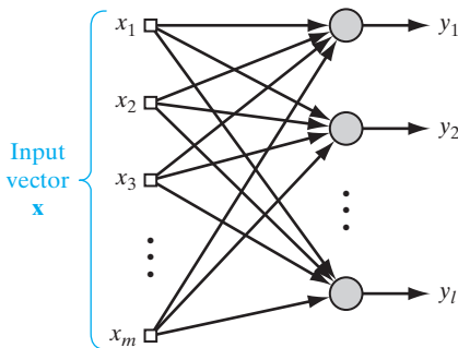
FIGURE 8.7 Feedforward network with a single layer of computational nodes.
