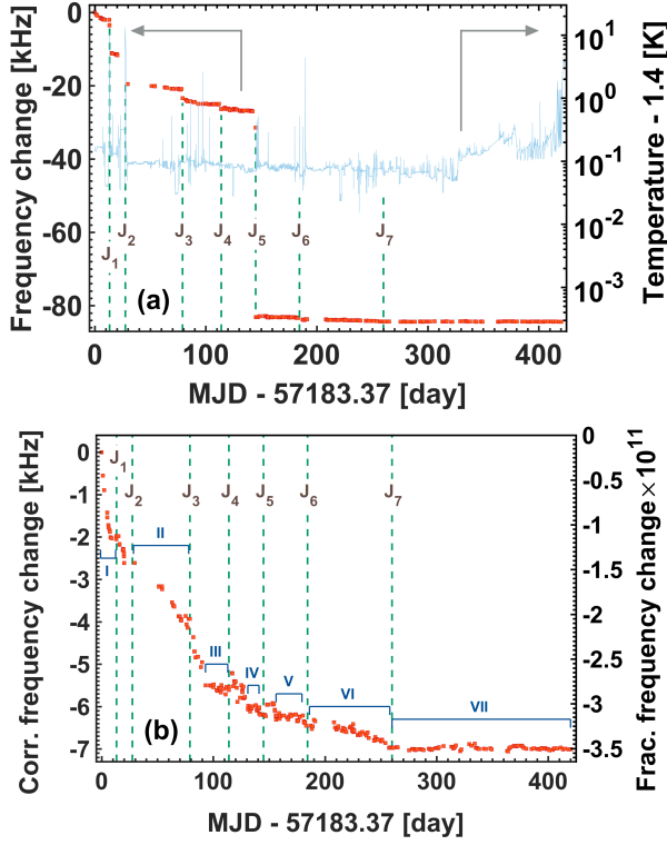
FIG. 2: (Color online). (a): Variation \Delta f_{res} of the optical frequency of the silicon resonator (left scale) and its temperature (right scale) over time. During intervals I - VI, the Pound-Drever-Hall locking technique was used. The shown data of interval VII was obtained using the frequency scan technique. Time zero corresponds to the first measurement, performed four days after reaching base temperature (1.5 K). (b): Corrected Si resonator frequency change, obtained by removing frequency jumps that occurred at J_1, \dots, J_6 .
