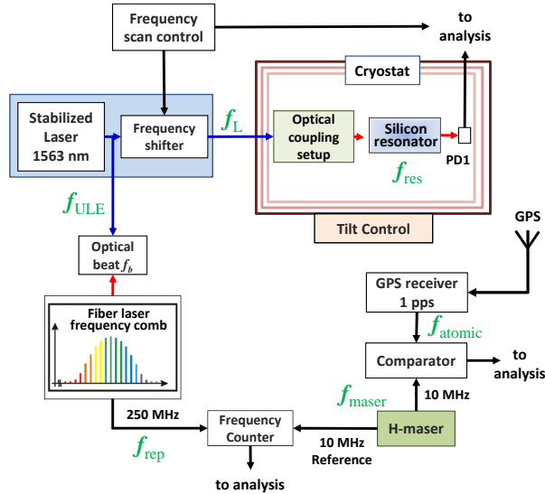
FIG. 1: (Color online). Principle of the experiment. The optical resonance frequency f_{res} of a silicon resonator is compared with a radiofrequency f_{maser} provided by a hydrogen maser. This is done via the intermediary of a laser whose wave of frequency f_L interrogates the resonator and is also measured by an optical frequency comb (pulse repetition rate f_{rep} ). The maser frequency is itself compared with a 1-Hz signal ( f_{atomic} ) obtained from GPS satellites.
