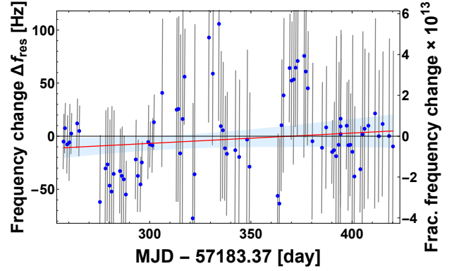
FIG. 3: (Color online). Resonator optical frequency variation \Delta f_{res} , corrected for maser drift, during time interval VII, defined in Fig. 2. Each data point (blue) is the average frequency value obtained during a measurement interval i . The bars indicate the range \pm twice the standard deviation of each data set i . Red line: time-linear fit, exhibiting a drift rate D_{res-atomic} = 5.9 \times 10^{-21}/s ; blue shaded area: 2\sigma uncertainty range of the time-linear fit. Zero ordinate value is defined as the mean of the data points.
