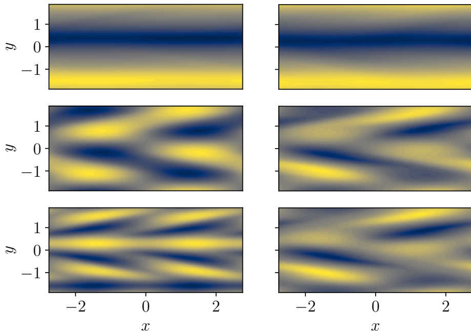
Figure 3: Streamwise velocity on a plane midway between the two walls for the DMD modes corresponding to the eigenvalue spectra reported in figure 2. The neutral mode and the first and second harmonics are shown. (Left) T_w = T_\omega , (right) T_w = T_\omega/4 .
