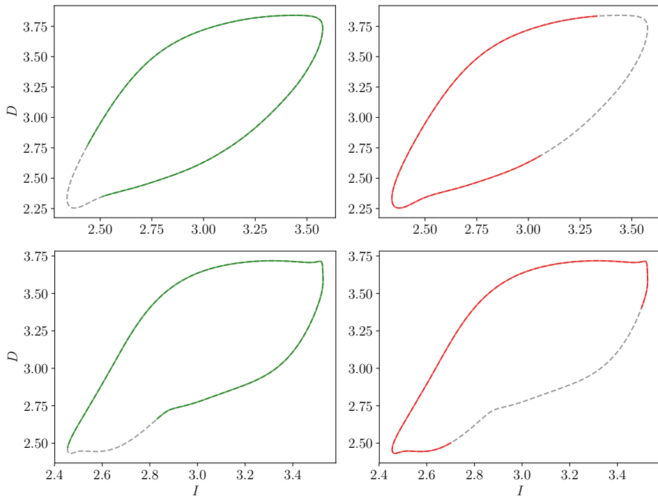
Figure 9: “Best” (left, in green) and “worst” (right, in red) locations for a DMD time window of length T_w = 60 as measured by the difference in predicted period from that of the true UPO, |T_g - T_w|/T_w , visualised in a two-dimensional projection of energy production against dissipation (both normalized by their values in laminar flow). The computations are performed on the UPOs themselves, and the full UPO is shown in dashed grey. The predicted period T_g = 2\pi/\omega_f , where \omega_f was computed from the first two harmonics. (Top) background UPO has period T_w = 85.60 . (Bottom) background UPO has period T_w = 94.76 .
