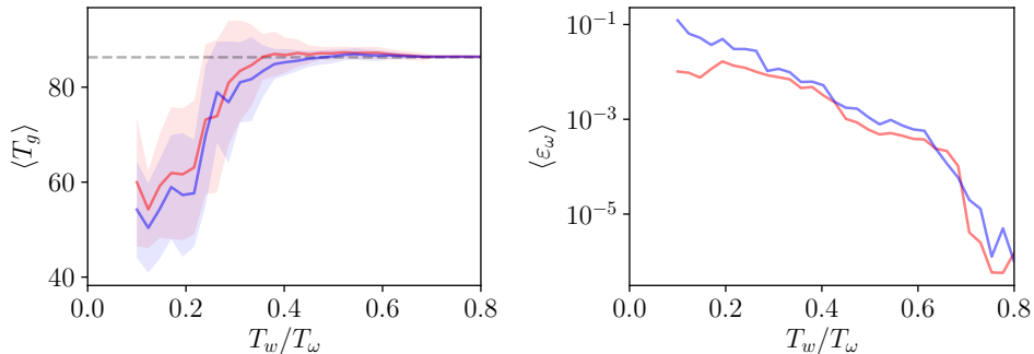
Figure 4: (Left) Average predicted period T_g = 2\pi/\omega_f of the edge state UPO as a function of observation window length using estimates based on two (red) and three (blue) harmonics. For each value of T_w , averaging is performed over sets of continuous time windows with start times separated by \Delta t_s = 5 . Shaded regions identify \pm 1 sample standard deviation. The horizontal dashed line identifies the true period T_\omega = 86.4 . (Right) ‘‘Quality’’ of the guessed period as determined by equation (2.8).
