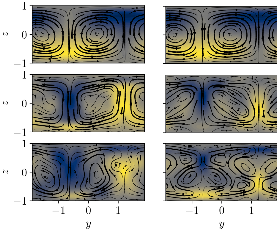
Figure 7: As figure 6, but now showing the streamwise-averaged streamwise velocity (contours) and the streamwise average y - z streamfunction (lines and arrows).
