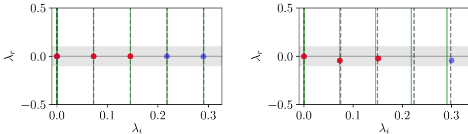
Figure 2: DMD eigenvalues obtained from observations on the “edge trajectory” described in the text. (Left) Observation window length matches the period of the edge UPO, T_w = T_\omega . (Right) Observation window is a quarter of the UPO period, T_w = T_\omega/4 . Green lines identify integer multiples of the fundamental frequency of the nearby UPO, 2\pi/T_\omega . Dashed black lines correspond to the fundamental frequency estimated from the first two harmonics (highlighted red) in the DMD via equation (2.8). The shaded region indicates a threshold \lambda_r^{\max} = 0.1 . In both calculations \delta t = 1 , M = 50 .
