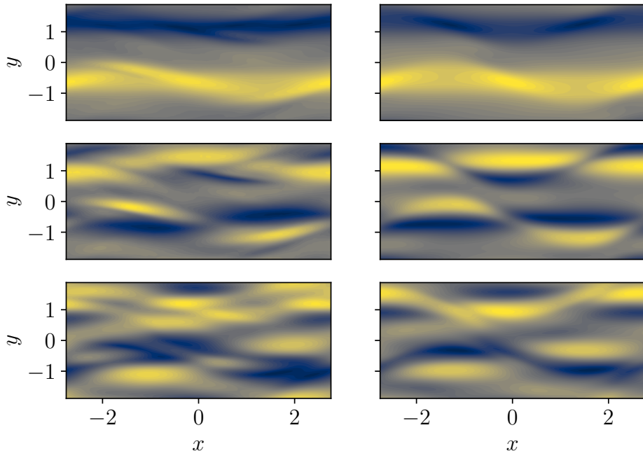
Figure 6: Contours of (the real part of) the streamwise velocity for the first three DMD modes for (left) the time window T_w = 60 starting at t_s = 780 (see Table 1) and (right) the converged UPO with period T_w = 71.83 . In both cases, the number of snapshot pairs is M = 100 , with \delta t = 1 .
