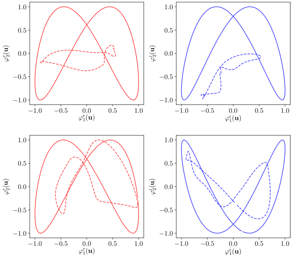
Figure 8: Real and imaginary components of approximate Koopman eigenfunctions, \varphi = \varphi^r + i\varphi^i , corresponding to the eigenvalues \lambda_1 \approx i\omega_f and \lambda_2 \approx 2i\omega_f , obtained in DMD applied to a converged UPO (solid lines) and the fixed turbulent window T_w = 60 that converged to that same UPO (dashed lines). In both cases the eigenfunction is evaluated along the UPO itself. (Top) The initial guess at t_s = 10 (see table 1) and the converged UPO T_w = 85.60 . (Bottom) The initial guess at t_s = 235 and the converged UPO T_w = 71.83 .
