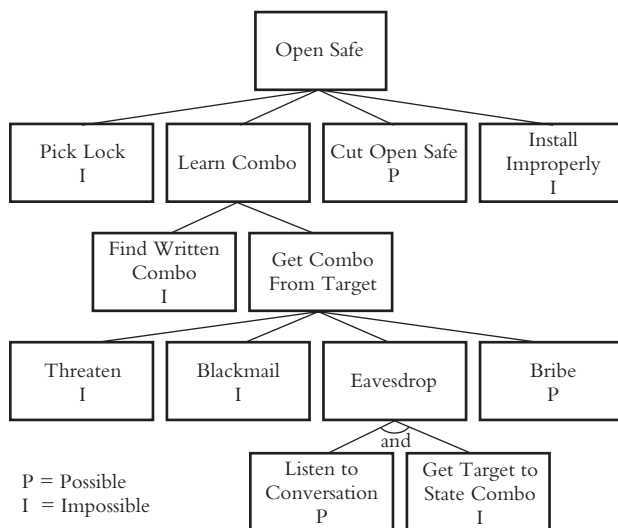
Figure 21.1 Attack nodes.
