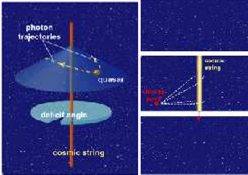
Figure 1.11: Cosmic strings affect surrounding spacetime by removing a small angular wedge, creating a conelike geometry (left). Space remains flat everywhere, but a circular path around the string encompasses slightly less than 360 degrees. The deficit angle is tiny, about 10^{-5} radian. To an observer, the presence of a cosmic string would be betrayed by its effect on the trajectory of passing light rays, which are deflected by an amount equal to the deficit angle. The resultant gravitational lensing reveals itself in the doubling of images of objects behind the string (right panel).
