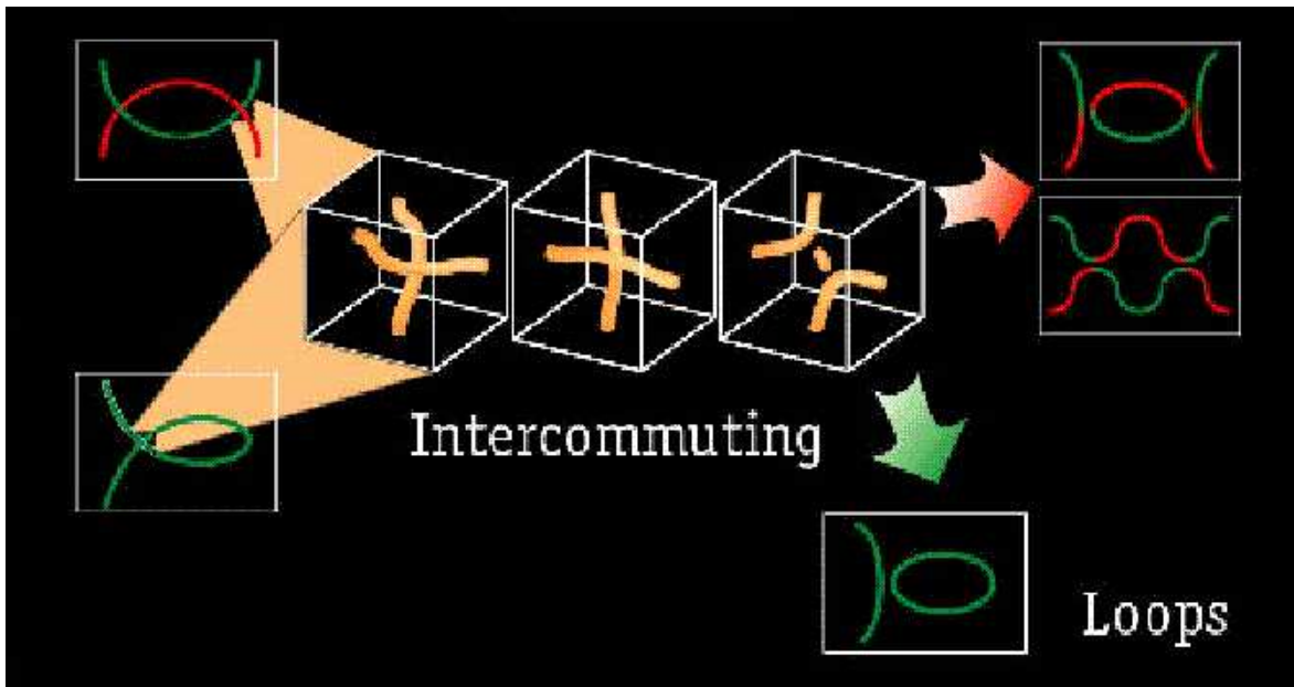
Figure 1.5: Global string interactions leading to loop formation. Whenever two string segments intersect, they reconnect or intercommute (green and red strings – upper part of the figure). Analogously, if a string intersects itself, it can break off a closed loop (green string – bottom part of the figure). In both cases, the interacting string segments first suffer a slight deformation (due to the long-range forces present for global strings), they subsequently fuse and finally exchange partners. A ephemeral unstable amount of energy in the form of a small loop remains in the middle where the energy is high enough to place the Higgs field in the false vacuum. It then quickly collapses, radiating away its energy. The situation is roughly the same for local strings, as simulations have shown.
