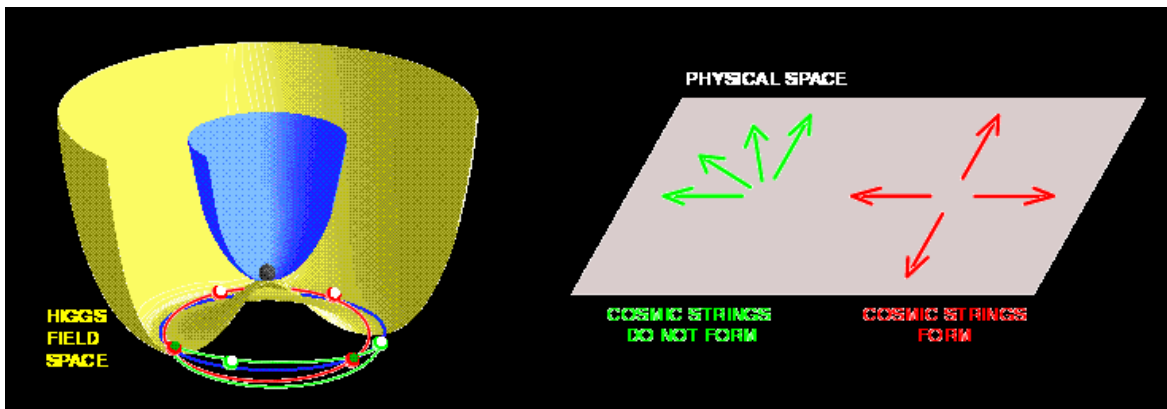
Figure 1.3: The complex scalar Higgs field evolves in a temperature-dependent potential V(\phi) . At high temperatures (violet surface) the vacuum expectation value of the field lies at the bottom of V . For lower temperatures, the potential adopts the “Mexican hat” form (yellow surface) and the field spontaneously chooses one amongst the new available (degenerate) lowest energy states (the violet circle along the valley of the hat). This isolates a single value/direction for the phase of the field, spontaneously breaking the symmetry possessed by the system at high energies. Different regions of the universe, with no causal connection, will end up having arbitrarily different directions for the field (arrows on the right). As separate regions of broken symmetry merge, it is not always possible for the field orientations to match. It may happen that a closed loop in physical space intersects regions where the Higgs phase varies from 0 to 2\pi (red arrows, corresponding to the red dashed-line on the left panel). In that situation, a cosmic string will pass somewhere inside the loop. On the contrary, green arrows (and green dashed-line on the left panel) show a situation where no string is formed after the phase transition.
