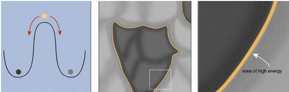
Figure 1.2: In a simple model of symmetry breaking, the initial symmetric ground state of the Higgs field (yellow dot) can fall into the left- or right-hand valley of a double-well energy potential (light and dark dots). In a cosmic phase transition, regions of the new phase appear randomly and begin to grow and eventually merge as the transition proceeds toward completion (middle). Regions in which the symmetry has broken the same way can coalesce, but where regions that have made opposite choices encounter each other, a topological defect known as a domain wall forms (right). Across the wall, the Higgs field has to go from one of the valleys to the other (in the left panel), and must therefore traverse the energy peak. This creates a narrow planar region of very high energy, in which the symmetry is locally unbroken.
