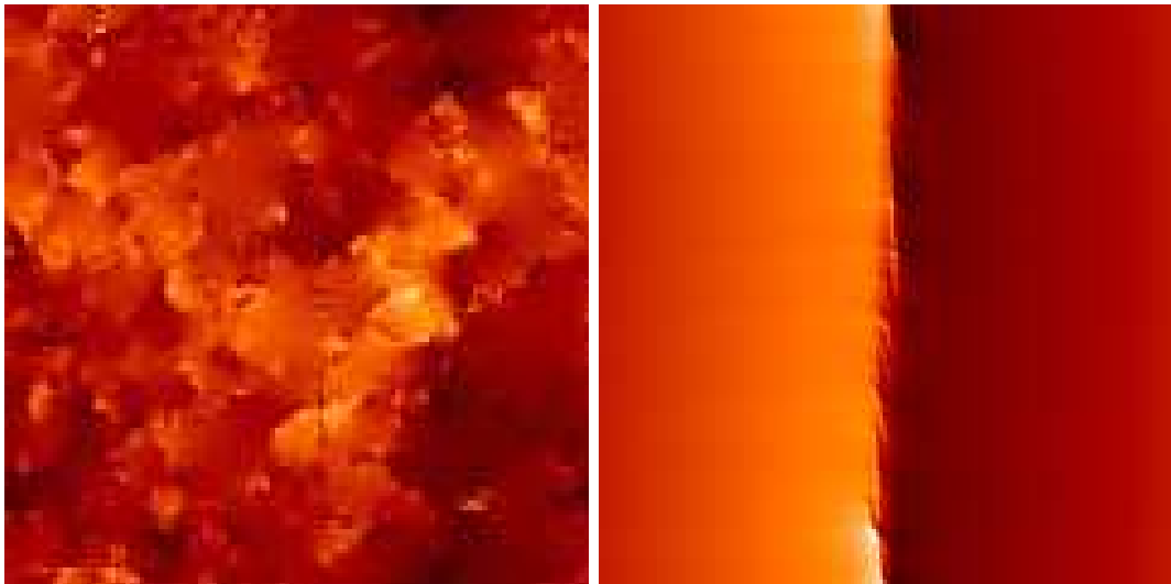
Figure 1.13: The Kaiser-Stebbins effect for cosmic strings. A string network evolves into a self-similar scaling regime, perturbing matter and radiation during its evolution. The effect on the CMB after recombination leads to distinct steplike discontinuities on small angular scales that were first studied by Kaiser & Stebbins [1984]. The left panel shows a simulated patch of the sky that fits in one of the pixels of the COBE experiment. Hence, higher resolution observatories are needed in order to detect strings. The right panel shows a patch on the CMB sky of order 20' across. However, recent studies indicate that this clean tell-tale signal gets obscured at subdegree angular scales due to the temperature fluctuations generated before recombination. [Magueijo & Ferreira 1997].
