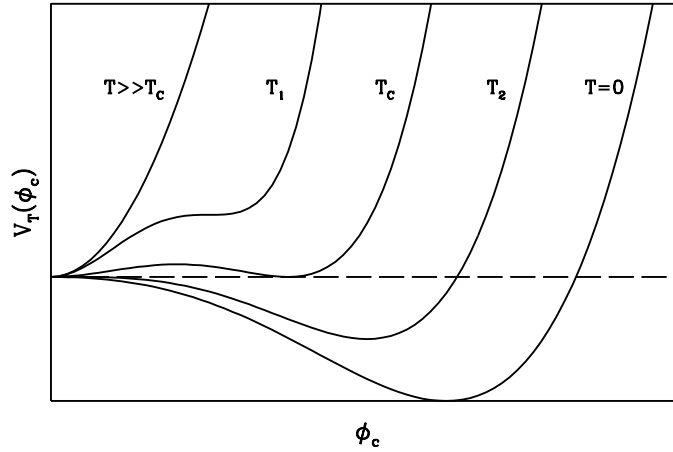
Figure 1.1: Temperature-dependent effective potential for a first-order phase transition for the Higgs field. For very high temperatures, well above the critical one T_c , the potential possesses just one minimum for the vanishing value of the Higgs field. Then, when the temperature decreases, a whole set of minima develops (it may be two or more, discrete or continuous, depending of the type of symmetry under consideration). Below T_c , the value \phi = 0 stops being the global minimum and the system will spontaneously choose a new (lower) one, say \phi = \eta \exp(i\theta) (for complex \phi ) for some angle \theta and nonvanishing \eta , amongst the available ones. This choice signals the breakdown of the symmetry in a cosmic phase transition and the generation of random regions of conflicting field orientations \theta . In a cosmological setting, the merging of these domains gives rise to cosmic defects.
