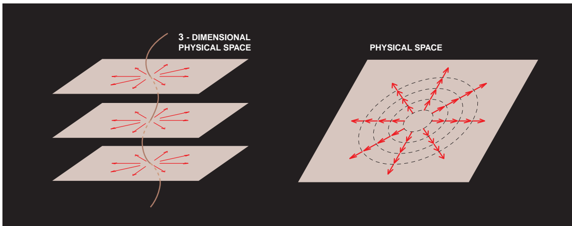
Figure 1.4: We can now extend the mechanism shown in the previous figure to the full three-dimensional space. Regions of the various planes that were traversed by strings can be superposed to show the actual location of the cosmic string (left panel). The figure on the right panel shows why we are sure a string crosses the plane inside the loop in physical space (the case with red arrows in the previous figure). Continuity of the field imposes that if we gradually contract this loop the direction of the field will be forced to wind “faster”. In the limit in which the loop reduces to a point, the phase is no longer defined and the vacuum expectation value of the Higgs field has to vanish. This corresponds to the central tip of the Mexican hat potential in the previous figure and is precisely the locus of the false vacuum. Cosmic strings are just that, narrow, extremely massive line-like regions in physical space where the Higgs field adopts its high-energy false vacuum state.
