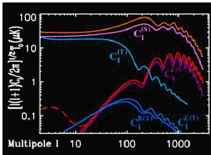
Figure 1.17: CMB Polarization for two different models. Red and orange (unlabeled) curves are the angular spectra derived for a \Lambda CDM model, both with (red dashed line) and without (red full line) reionization. The temperature anisotropy spectrum from scalar perturbations (proportional to [C_\ell]^{1/2} , orange curve) is virtually unchanged for both ionization histories. The polarization spectrum ( \propto [C_\ell^{E(S)}]^{1/2} , red curves), although indistinguishable for \ell \gtrsim 20 , dramatically changes for small \ell 's; in this model the Universe is reionized suddenly at low redshift with optical depth \tau_c = 0.05 . Blue and violet curves represent a SCDM model but with a high tensor-mode amplitude, T/S=1 at the quadrupole ( \ell = 2 ) level, with scale-invariant spectral indices n_S = 1 and n_T = 0 . Separate scalar (noted C_\ell^{(S)} ) and tensor ( C_\ell^{(T)} ) contributions to temperature anisotropies are shown (top curves). Scalar modes only generate E-type polarization ( C_\ell^{E(S)} ), which is smaller than the corresponding red curve of the \Lambda CDM model both due to differences in the models (notably \Lambda \neq 0 for the red curves) and due to the influence of tensors on the normalization at small \ell . E- and B-type polarization from tensor modes are also shown, respectively C_\ell^{E(T)} and C_\ell^{B(T)} . Model spectra were computed with CMBFAST and are normalized to \delta T_{\ell=10} = 27.9\mu\text{K} .
