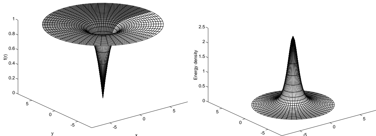
Figure 1.6: Higgs field and energy profiles for Goto–Nambu cosmic strings. The left panel shows the amplitude of the Higgs field around the string. The field vanishes at the origin (the false vacuum) and attains its asymptotic value (normalized to unity in the figure) far away from the origin. The phase of the scalar field (changing from 0 to 2\pi ) is shown by the shading of the surface. In the right panel we show the energy density of the configuration. The maximum value is reached at the origin, exactly where the Higgs is placed in the false vacuum. [Hindmarsh & Kibble, 1995].
