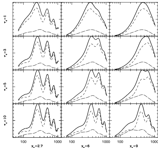
Figure 1.15: The predictions of the toy model of Magueijo, et al. [1996] for different values of parameters x_c , the coherence length, and \tau_c , the coherence time. x_c \propto \eta/\lambda_c(\eta) , where \eta is the conformal time and \lambda_c(\eta) is the correlation length of the network at time \eta . One can obtain oscillations in the CMB power spectrum by fixing either one of the parameters and varying the other.
