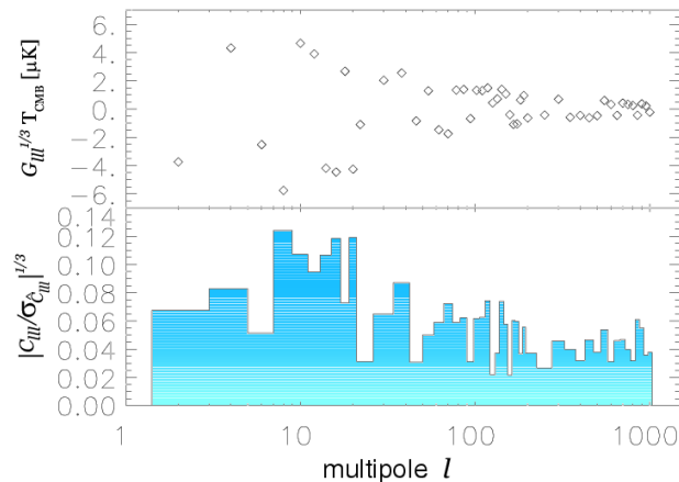
Figure 1.16: The CMB angular bispectrum in the ‘diagonal’ case ( G_{ll}^{1/3} ) from wiggly cosmic strings in a spatially flat model with cosmological parameters \Omega_{\text{CDM}} = 0.3 , \Omega_{\text{baryon}} = 0.05 , \Omega_{\Lambda} = 0.65 , and Hubble constant H = 0.65 \text{ km s}^{-1} \text{ Mpc}^{-1} [upper panel]. In the lower panel we show the ratio of the signal to theoretical noise |C_{ll}/\sigma_{C_{ll}}|^{1/3} for different multipole indices. Normalization follows from fitting the power spectrum to the BOOMERANG and MAXIMA data.
