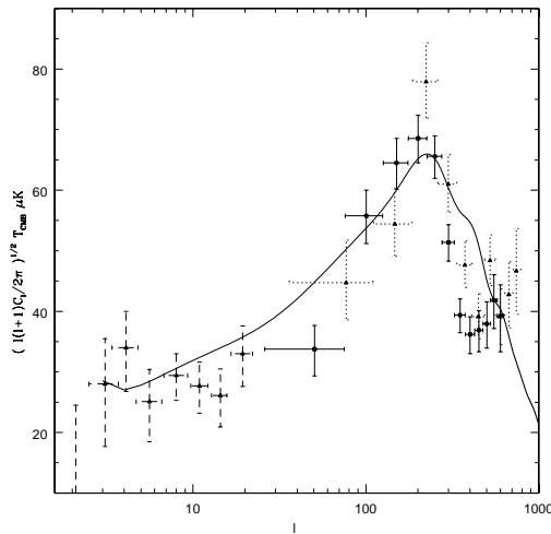
Figure 1.14: The CMB power spectrum produced by the wiggly string model of [Pogosian & Vachaspati, 1999] in a closed universe with \Omega_{\text{total}} = 1.3 , \Omega_{\text{baryon}} = 0.05 , \Omega_{\text{CDM}} = 0.35 , \Omega_{\Lambda} = 0.9 , and H_0 = 65 \text{ km s}^{-1}\text{Mpc}^{-1} [Pogosian, 2000].
