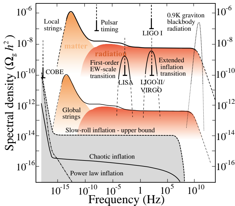
Figure 1.22: A summary of the spectral density versus frequency for various potential sources of a stochastic gravitational wave background. Included in this busy plot are the amplitudes of GW from different types of inflationary scenarios, from a first-order electroweak phase transition, and from both gauge and global cosmic strings, also including the primordial 0.9 K blackbody spectrum of gravitons. [Battye & Shellard, 1996].
