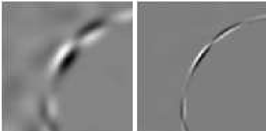
Figure 1.19: Simulations for the B field in the case of a circular loop. The angular size of the figure is 50' \times 50' . The resolution is 5' (left) and 1.2' (right). The discontinuity in the B field is sharper the better the resolution. Weak lensing of CMB photons passing relatively apart from the position of the string core are apparent as faint patches outside of the string loop on the left panel. [Benabed & Bernardeau 2000].
