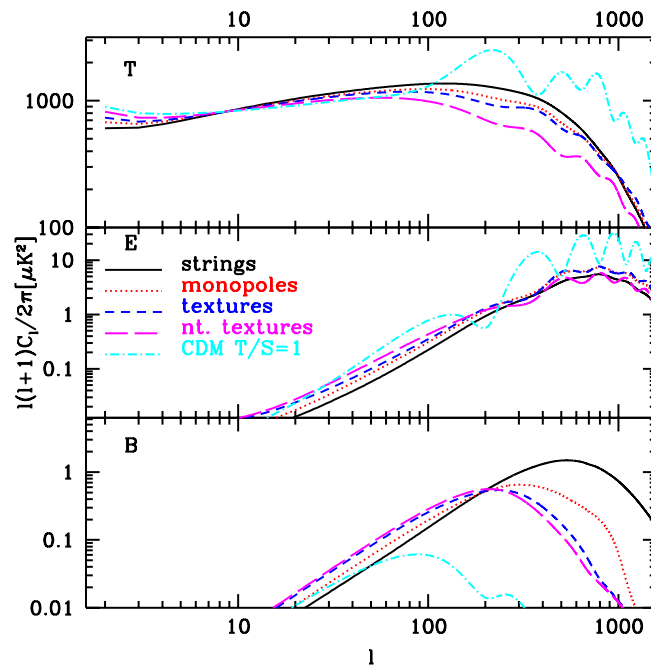
Figure 1.18: Power spectra of temperature ( T ), electric type polarization ( E ) and magnetic type polarization ( B ) for global strings, monopoles, textures and nontopological textures [taken from Seljak. et al. , 1997]. The corresponding spectra for a standard CDM model with T/S = 1 is also shown for comparison. B polarization turns out to be notably larger for all global defects considered if compared to the corresponding predictions of inflationary models on small angular scales.
