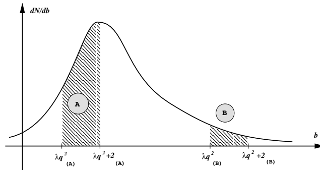
Figure 1.24: A possible way out of the vorton excess problem: a sketch of a distribution of loops with b \simeq N/Z , and vorton-forming intervals for different values of the electromagnetic correction \lambda q^2 to the vorton equation of state. It is clear that the actual number density of ensuing vortons, at most proportional to the shaded areas, will depend quite strongly on the location of this interval. Note also that this electromagnetic correction may reduce drastically the available phase space for vorton formation since the maximum of the dN/db distribution is usually assumed to be peaked around b = 1 . [Gangui, Peter & Boehm, 1998].
