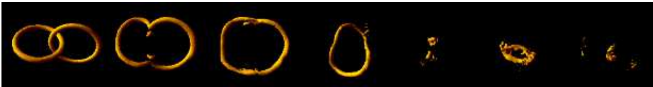
Figure 1.23: A series of snapshots from a two interlocked cosmic string loop decay process [courtesy of R. Battye and P. Shellard]. Loops disintegrate through the emission of (mainly gravitational) radiation. However, if endowed with currents, the loops may eventually reach equilibrium configurations (vortons) which will prevent their radiative decay. Such a population of vortons would jeopardize the so far successful standard model, unless it is produced at low enough energies.
