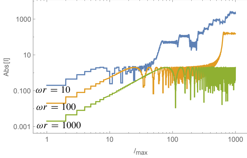
Figure 2. The partial wave sum (34) as a function of \ell_{\max} for \omega r = 10, 100, 1000 .
