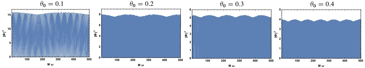
Figure 14. The power spectrum of the scattering wave with r_s = 7M . The amplitude of the modulation is \Delta I/I \sim 0.1 . The period of the modulation depends on the viewing angle \theta_0 .
